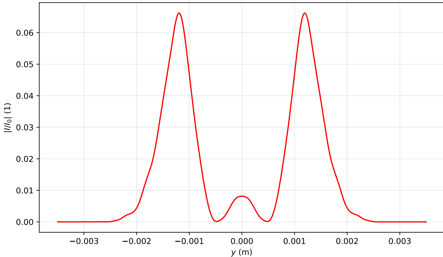
Intensity profile I(x=0, y, z=3.582)/I_0 , P_{in}=7.0P_{cr} , artificial time
